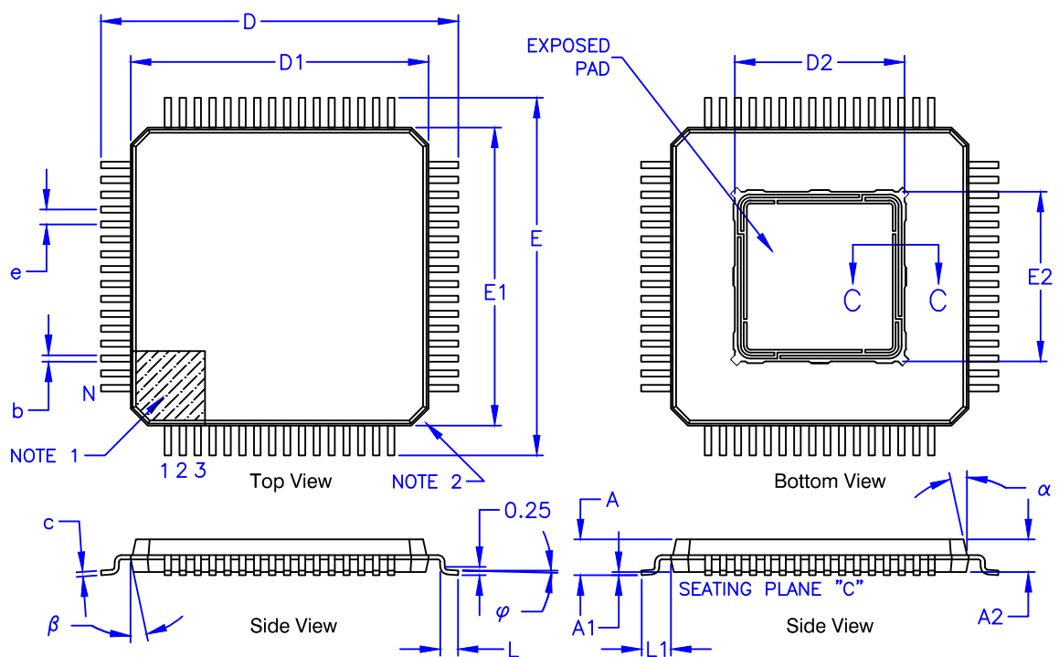
FIGURE 21-3: 64-TQFP-EP PACKAGE
