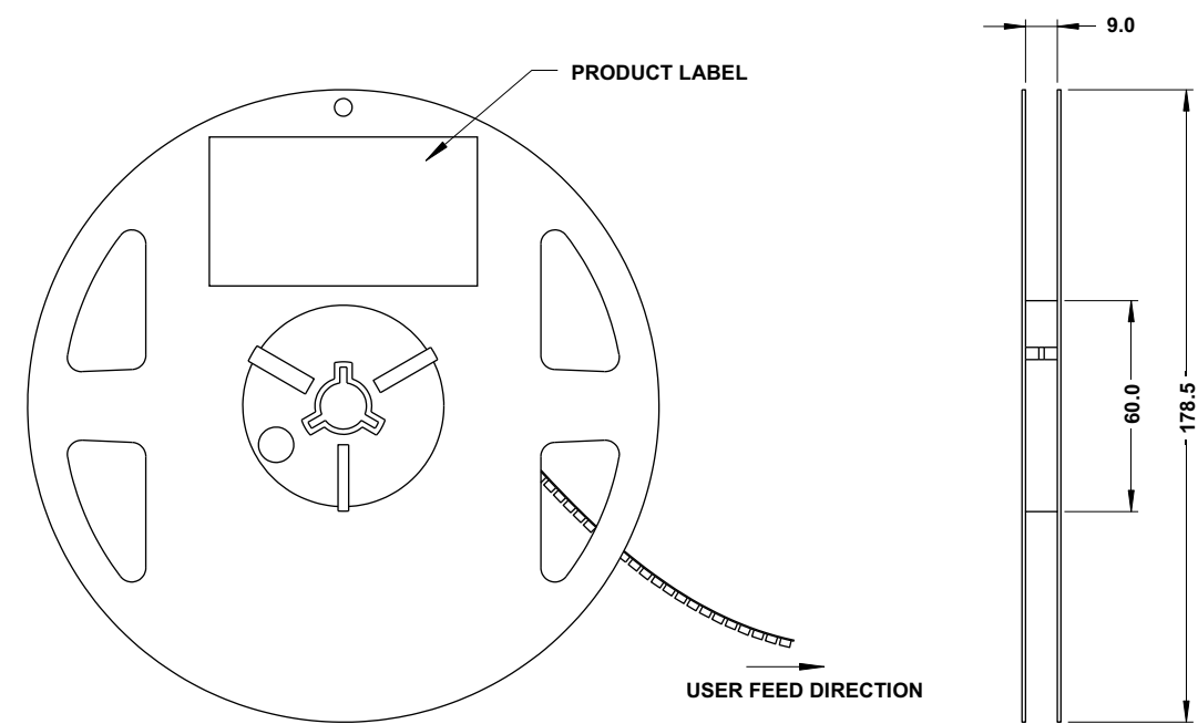
Figure 20 Reel Dimension
