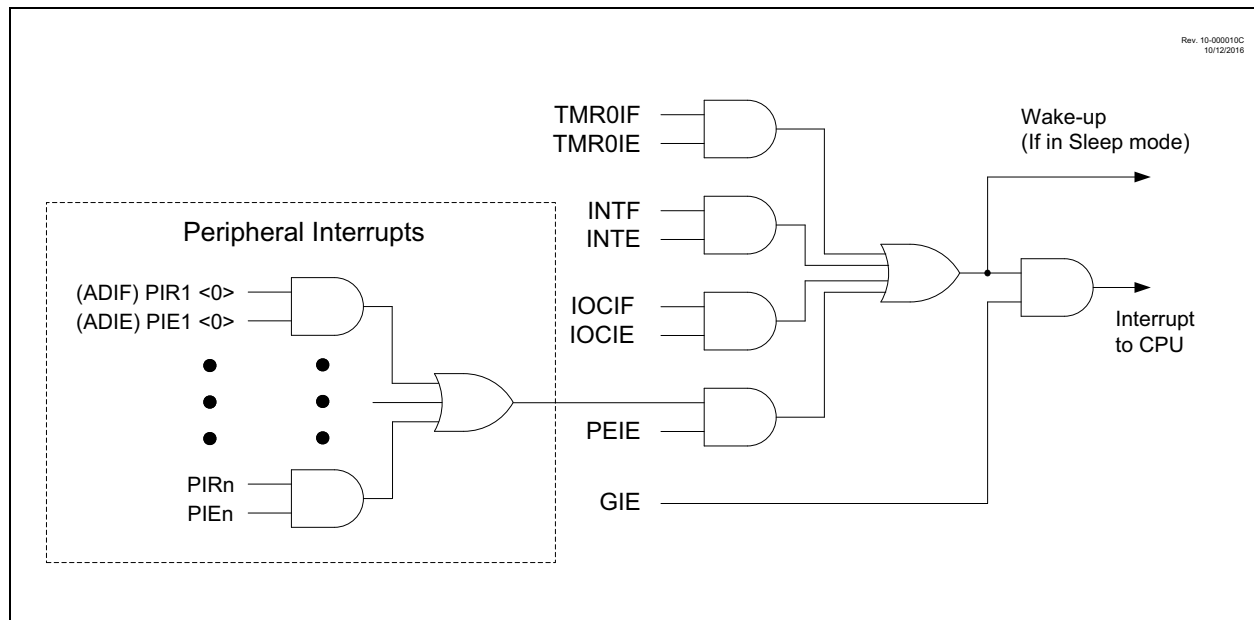
FIGURE 10-1: INTERRUPT LOGIC
