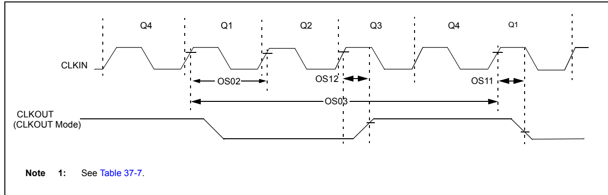
FIGURE 37-5: CLOCK TIMING
