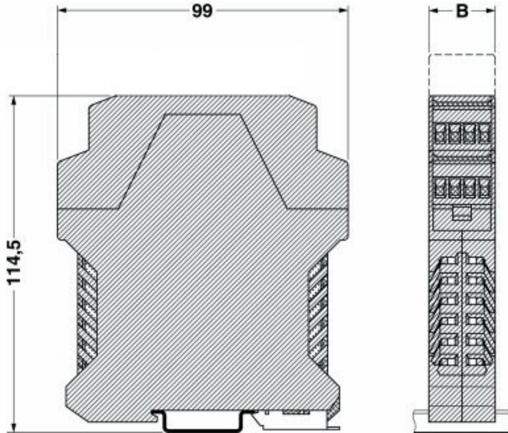
Dimensioned drawing
