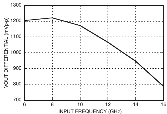
Output Differential Voltage vs. Frequency [1][3]
