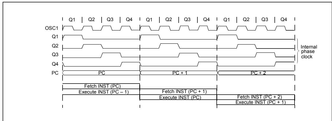
FIGURE 3-3: CLOCK/INSTRUCTION CYCLE
