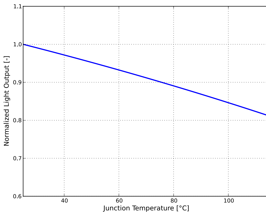
Figure 2a. Typical normalized light output vs. junction temperature for L130-xxxxxx1400001 at 60mA.
