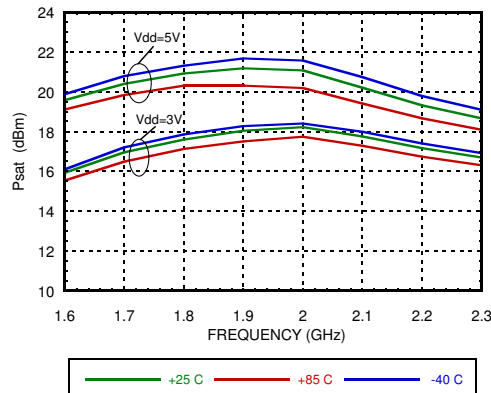
Psat vs. Temperature [1] [2]
