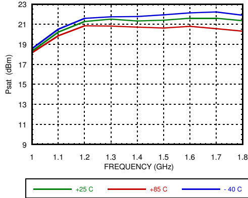
Psat vs. Temperature [1]
