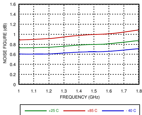
Noise Figure vs. Temperature [1]
