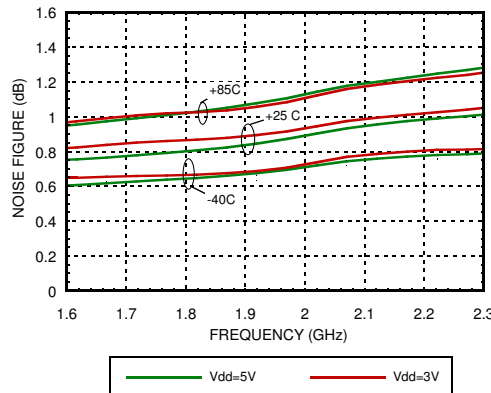
Noise Figure vs. Temperature [1] [2] [3]
