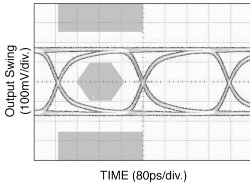
3.2Gbps Data
