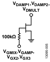
Figure 5. VGAMP1, VGAMP2, VGAMP, VGX2, VGX3 Interface
