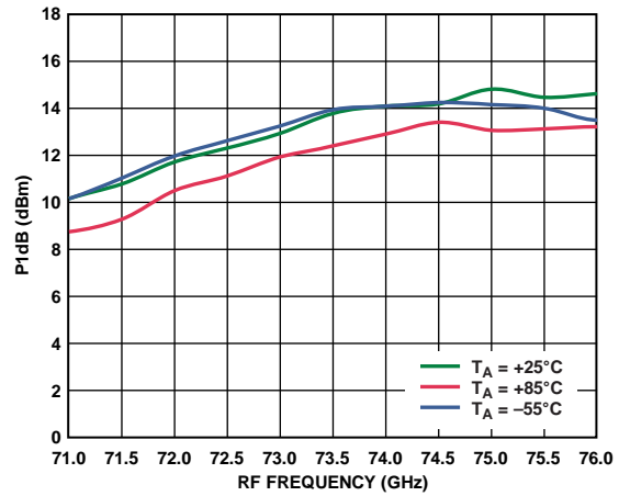
Figure 32. Input P1dB vs. RF Frequency at Various Temperatures, LO = 2 dBm, IF = 500 MHz, LSB
