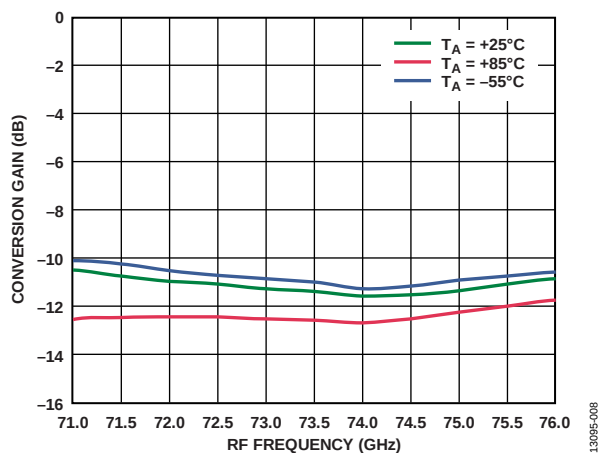
Figure 8. Conversion Gain vs. RF Frequency at Various Temperatures, IFIN = -8 dBm, LO = 2 dBm, IF = 1000 MHz, LSB
