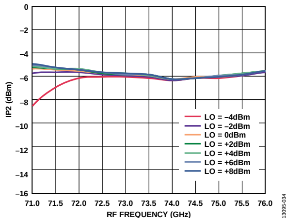
Figure 33. Input IP2 vs. RF Frequency at Various LO Powers, I_{FIN} = 5 \text{ dBm} , IF = 500 \text{ MHz} , LSB
