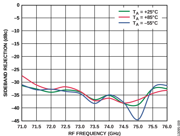
Figure 9. Sideband Rejection vs. RF Frequency at Various Temperatures, IFIN = -8 dBm, LO = 2 dBm, IF = 1000 MHz, LSB
