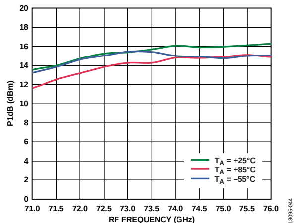
Figure 43. Input P1dB vs. RF Frequency at Various Temperatures, LO = 2 dBm, IF = 2000 MHz, LSB
