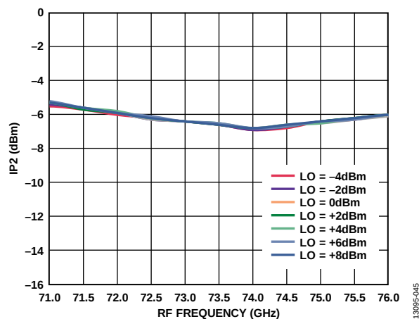
Figure 44. Input IP2 vs. RF Frequency at Various LO Powers, I_{FIN} = 5 dBm, IF = 2000 MHz, LSB
