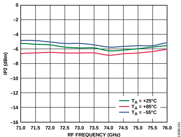
Figure 30. Input IP2 vs. RF Frequency at Various Temperatures, I_{FIN} = 5 \text{ dBm} , LO = 2 \text{ dBm} , IF = 500 \text{ MHz} , LSB
