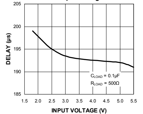
Output Turn-On Delay vs. Input Voltage
