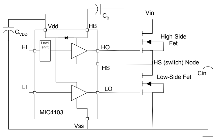
Figure 11. Synchronous Buck Converter Power Stage
