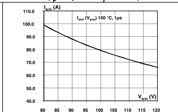
Figure 11. Reverse safe operating area ( t_p < 1 \mu s and T_j < 150 \text{ }^\circ\text{C} )
