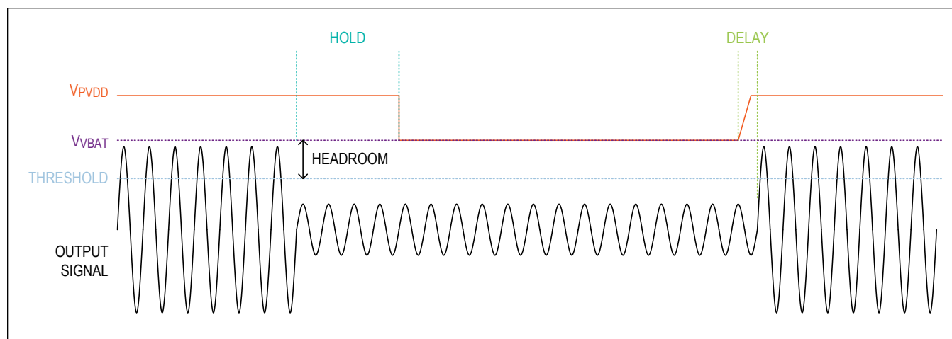
Figure 5. Boost Bypass
