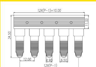
Dimensions - mm
