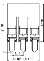
Dimensions - mm
