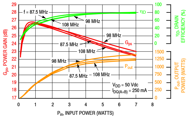
Figure 15. Power Gain, Drain Efficiency and CW Output Power versus Input Power and Frequency
