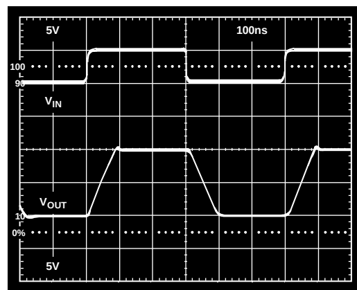
Figure 51. AD810 Driving a 1000 pF Load, Gain = +2, R_F = 750 \Omega , R_S = 11 \Omega , R_L = 10 k\Omega
