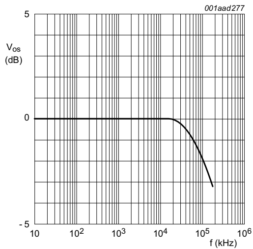
Fig 19. Frequency response
