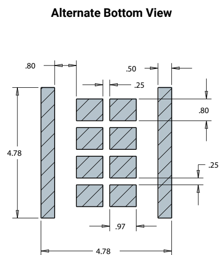
Recommended Stencil Pattern (Shaded Area is Open)
