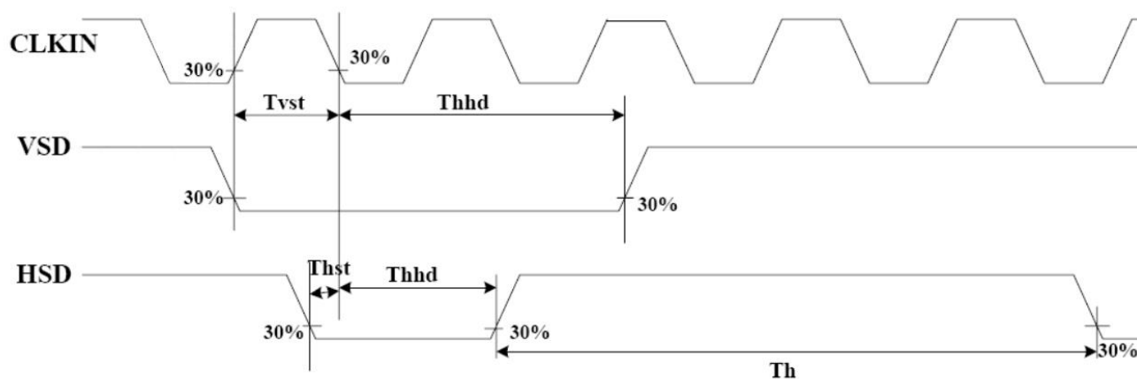
Figure 4: Clock input VSD/HSD timing diagram
