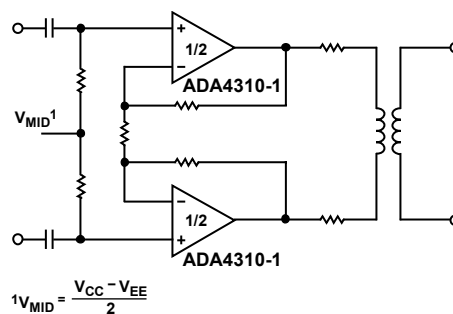
Figure 3. Typical PLC Driver Application
