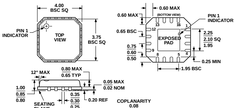
Figure 23. 16-Lead Lead Frame Chip Scale Package [LFCSP_VQ] 4 mm x 4 mm Body, Very Thin Quad (CP-16-4)
