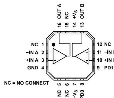
Figure 2. Thermally Enhanced, 4 mm \times 4 mm 16-Lead LFCSP_VQ
