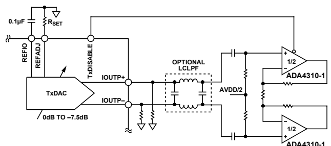
Figure 21. TxDAC Output Directly via Center-Tap Transformer
