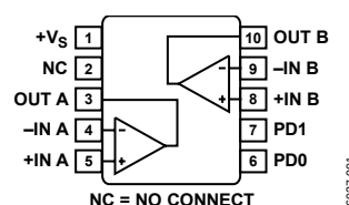
Figure 1. Thermally Enhanced, 10-Lead MINI_SO_EP
