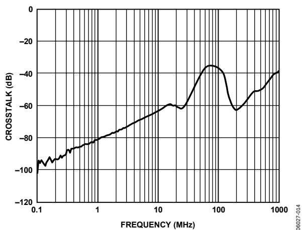
Figure 19. Crosstalk
