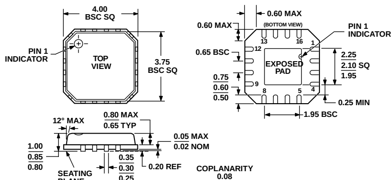
Figure 23. 16-Lead Lead Frame Chip Scale Package [LFCSP_VQ] 4 mm x 4 mm Body, Very Thin Quad (CP-16-4)
