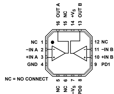
Figure 2. Thermally Enhanced, 4 mm \times 4 mm 16-Lead LFCSP_VQ
