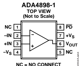
Figure 1. Single 8-Lead ADA4898-1 SOIC_N_EP (RD-8-1)
