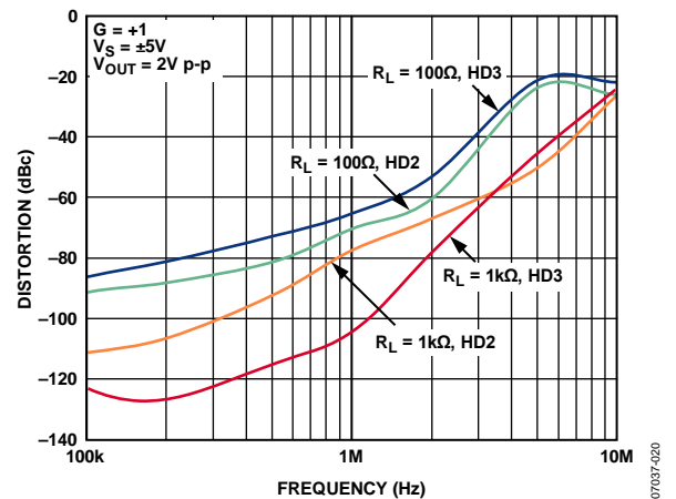
Figure 23. Harmonic Distortion vs. Frequency and Loads
