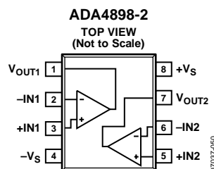
Figure 2. Dual 8-Lead ADA4898-2 SOIC_N_EP (RD-8-2)
