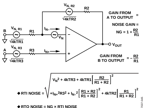
Figure 49. Op Amp Noise Analysis Model
