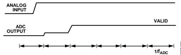
Figure 56. Step Change on Analog Input, Sinc 4 Filter
