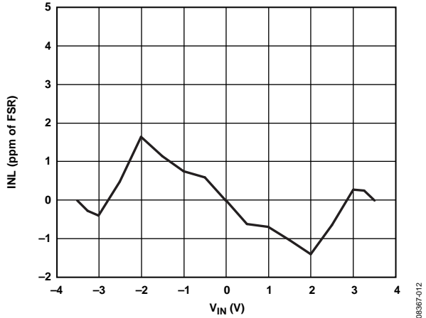
Figure 13. INL (Gain = 1)
