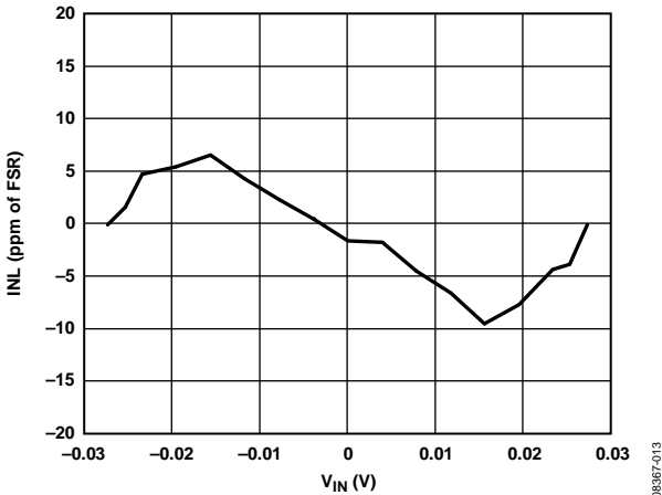
Figure 14. INL (Gain = 128)
