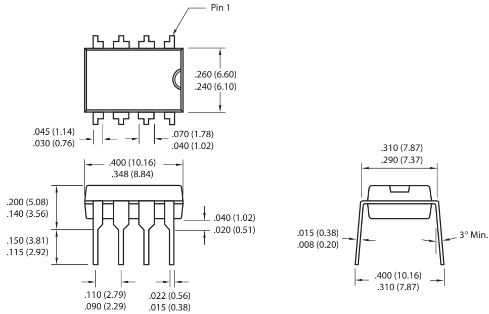
8-Pin Plastic DIP
