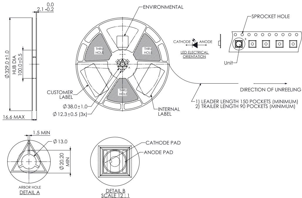
Figure 13. Reel dimensions for LUXEON V2.
