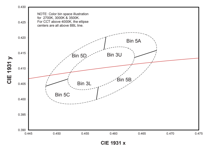
Figure 7. Color space definition for LUXEON V.
