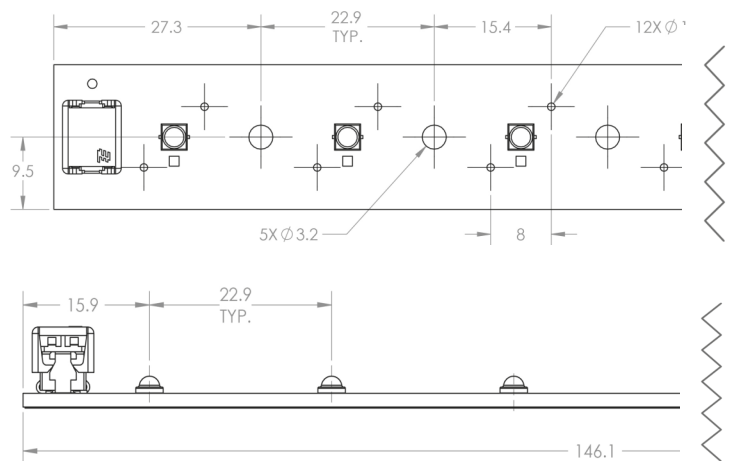
Linear 6 LED Array Dimensions: Length & Positioning
