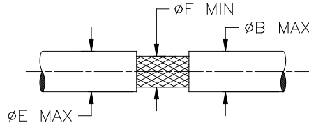
For terminators with pre-installed leads.
