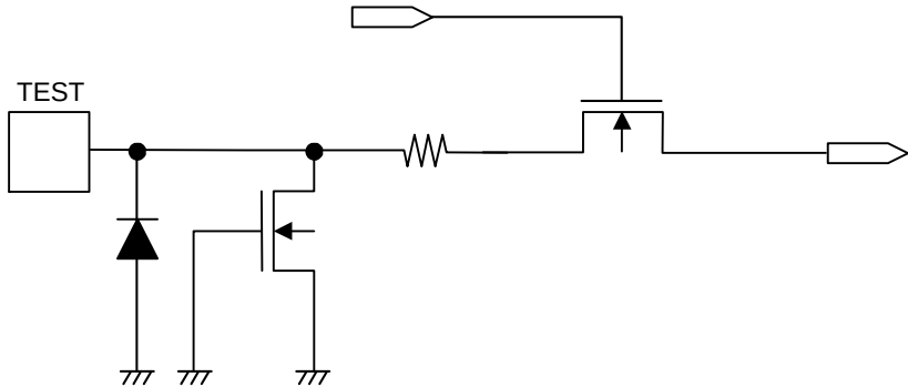
Figure 26 TEST Pin
