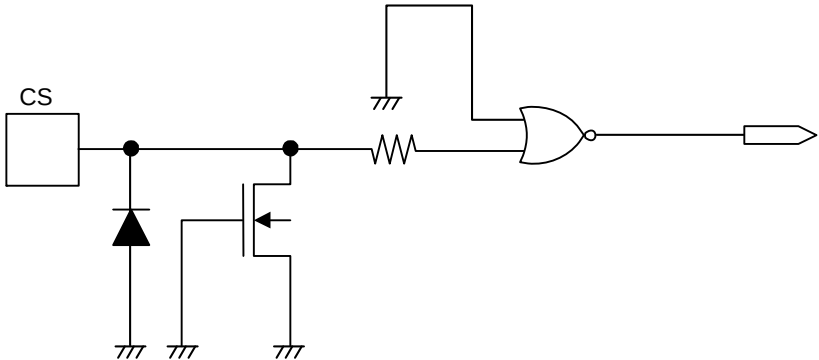
Figure 24 CS Pin
