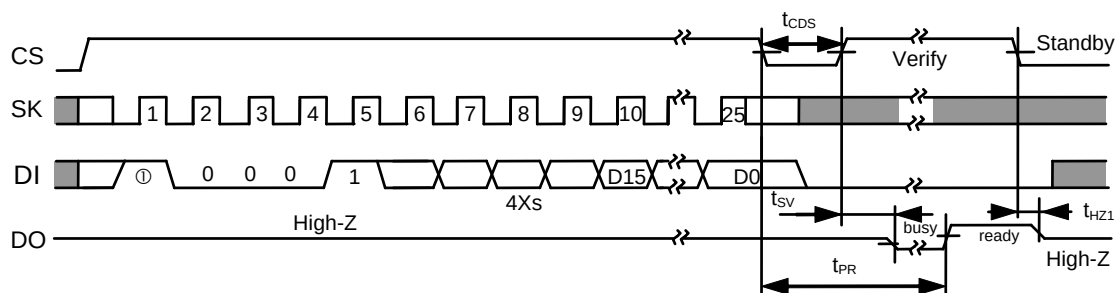
Figure 15 Chip Write Timing (S-93C46B)
