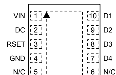
10-Pin 2mm x 2mm Thin MLF ® (MT) (Top View)
