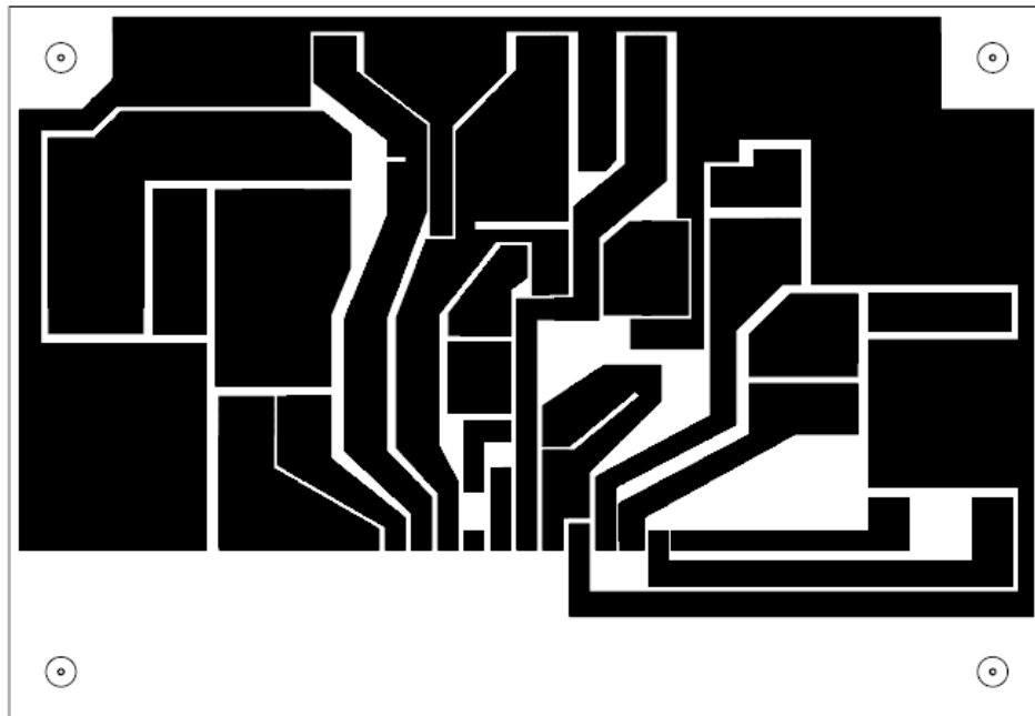
Figure 11. Top View
