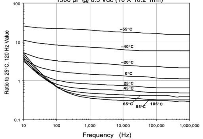
ESR vs. Temperature and Frequency 1500 \mu\text{F} @ 6.3 Vdc (10 X 10.2 mm)
