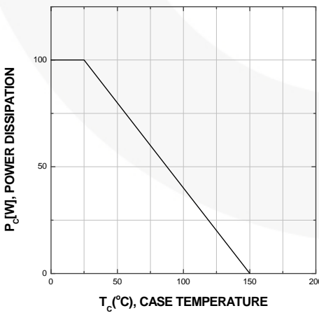
Figure 17. Power Derating
