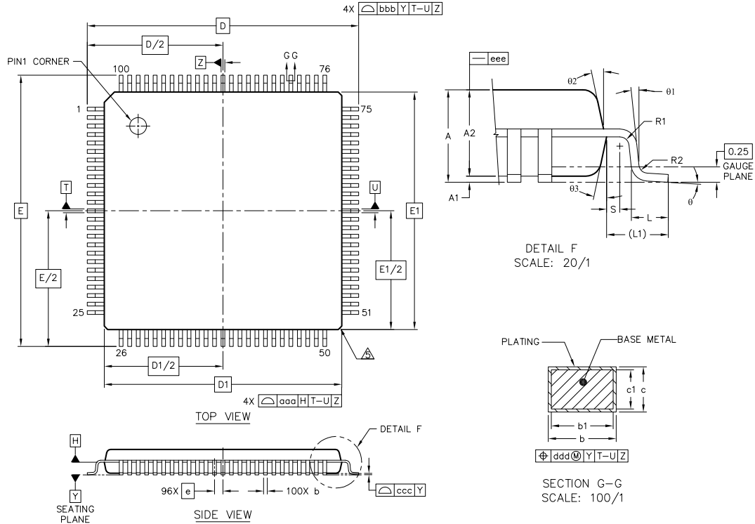
Figure 8.1. LQFP100
