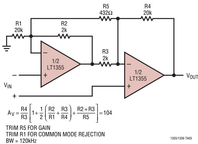
Instrumentation Amplifier
