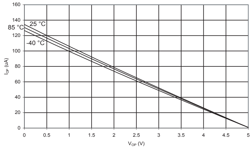
Figure 180. I/O Pin Pull-up Resistor Current vs. Input Voltage ( V_{CC} = 5V )
