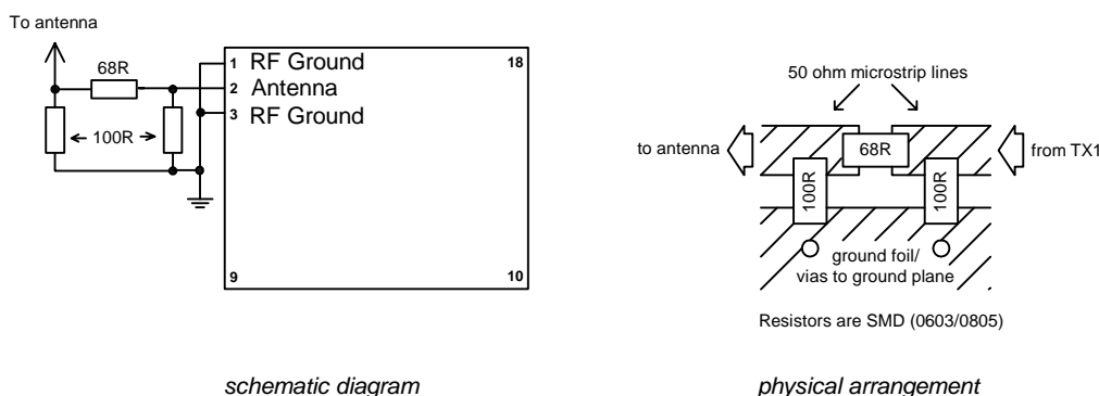
Figure 6: 10dB attenuator for BiM1 transceiver, BiM1T transmitter
