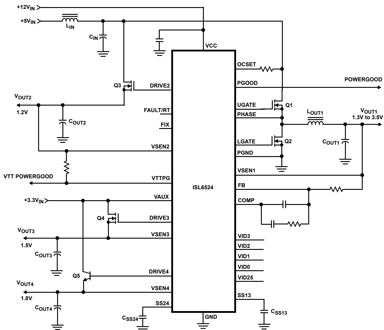
FIGURE 3. TYPICAL APPLICATION
