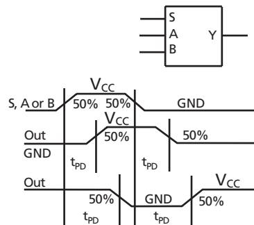
Figure 1-16 • C-Cell Delays
