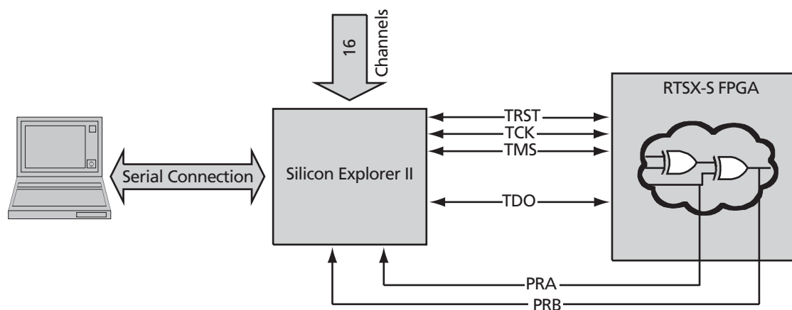
Figure 1-11 • Probe Setup
