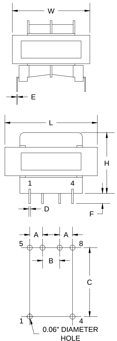
Board Layout
