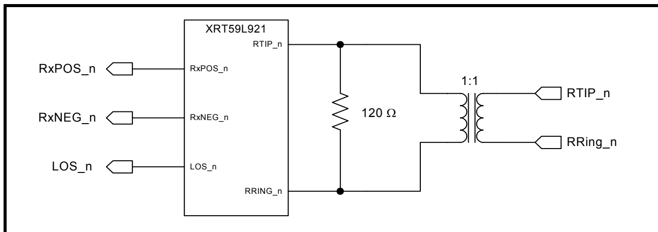
FIGURE 10. RECOMMENDED SCHEMATIC FOR INTERFACING THE RECEIVE SECTIONS OF THE XRT59L921 TO THE LINE FOR 120 \Omega APPLICATIONS (TRANSFORMER-COUPLING)
