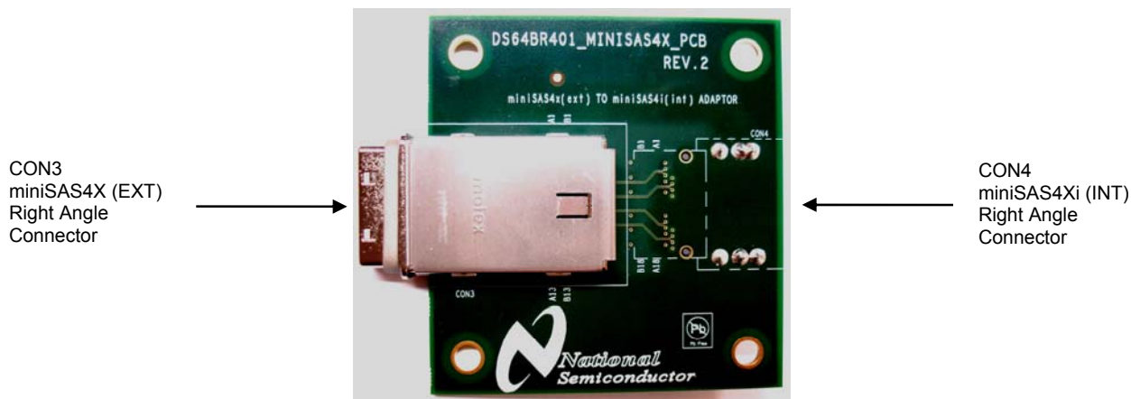
Figure 2. MiniSAS4X Connector Adaptor Board (EXT to INT)
