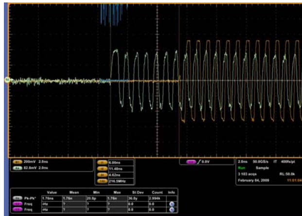
Idle to Active Response Time: ~ 4.6 ns
