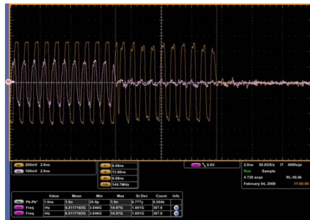
Active to Idle Response Time: ~ 6.7 ns
