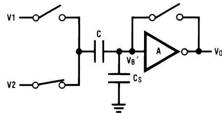
FIGURE 6. Sampled-Data Comparator
