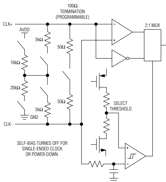
Figure 8. Simplified Clock Input Schematic
