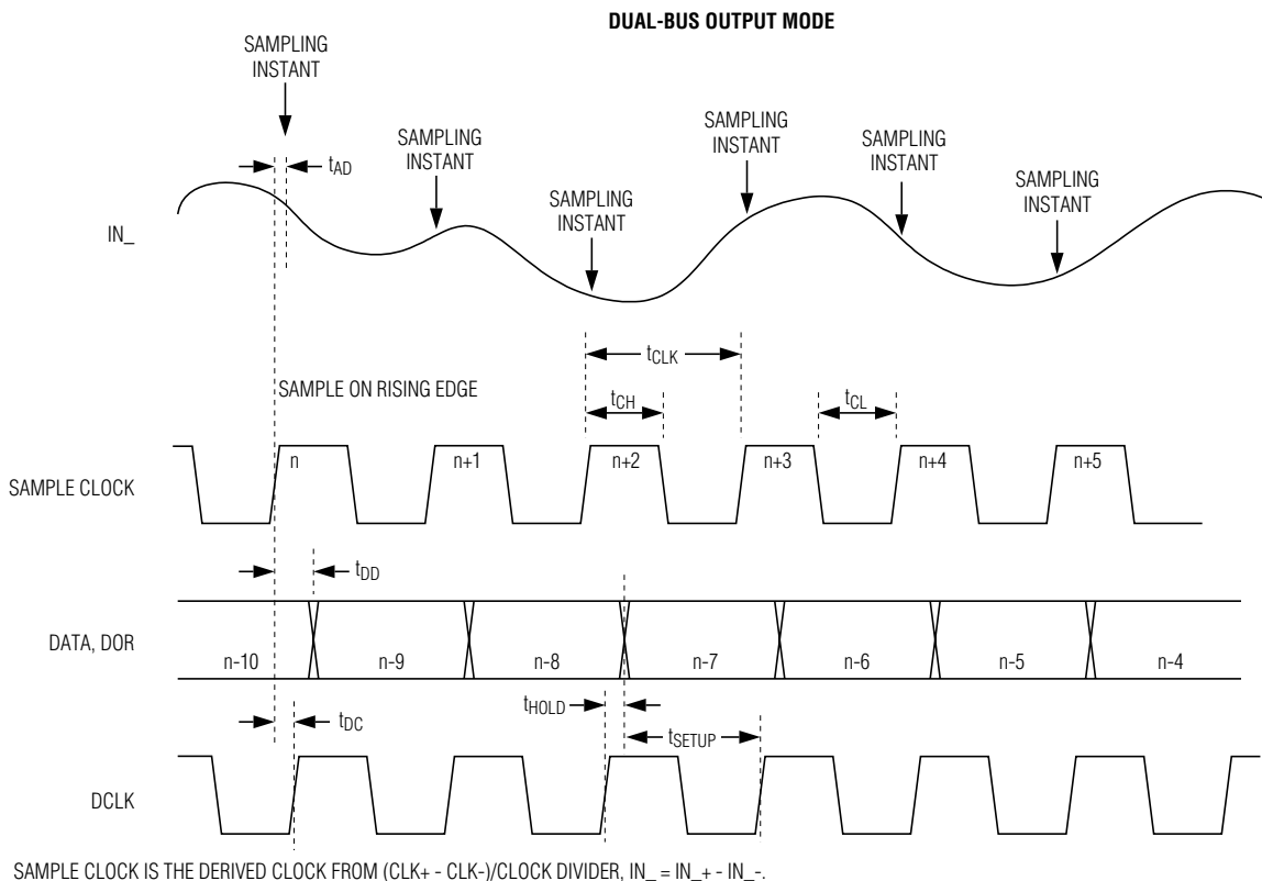
Figure 9. Dual-Bus Output Mode Timing
